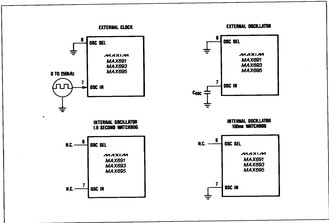
Figure 8. Oscillator Circuits
