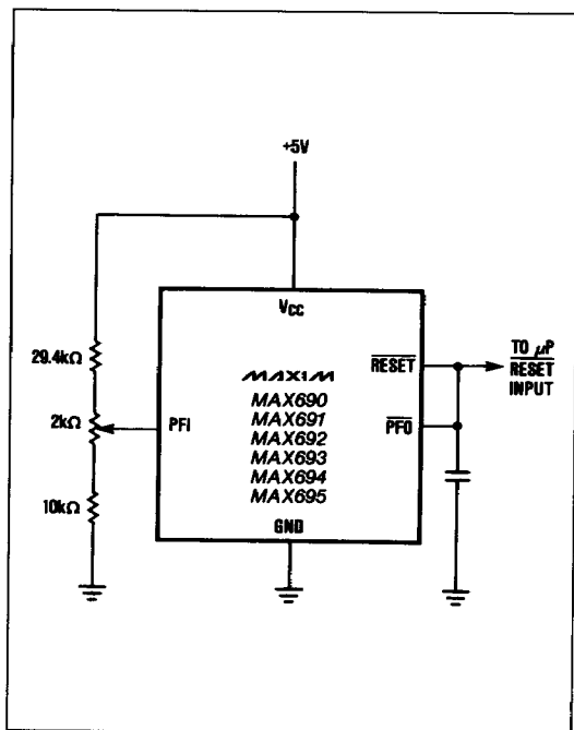
Figure 9. Externally Adjustable V_{CC} Reset Threshold
