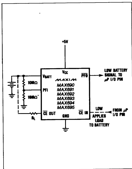
Figure 11. Backup Battery Monitor with Optional Test Load
