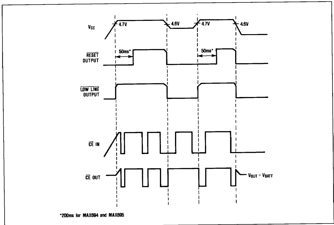
Figure 6. Reset Timing
