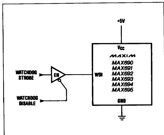
Figure 13. Disabling the Watchdog Under Program Control
