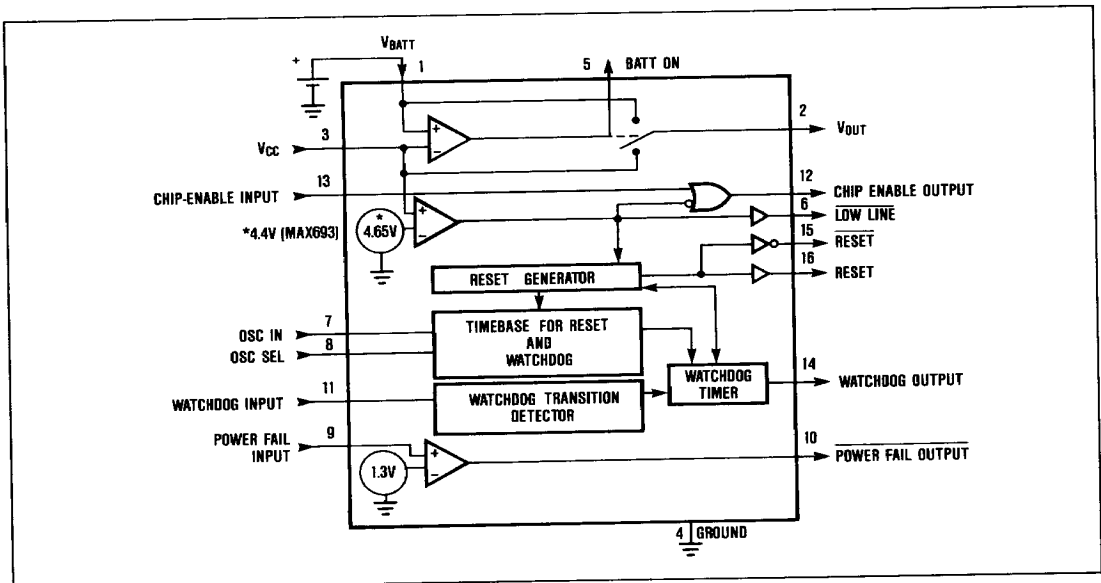
Figure 3. MAX691/693/695 Block Diagram
