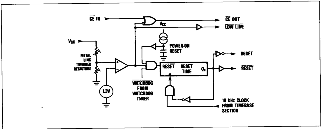
Figure 5. Reset Block Diagram
