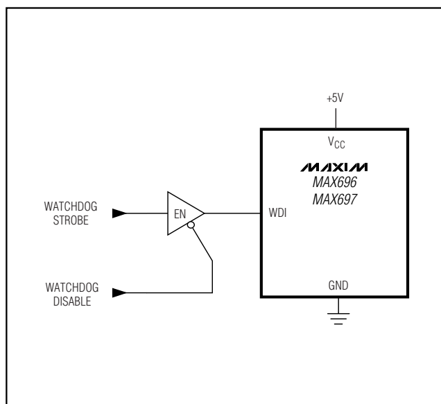
Figure 8. Disabling the Watchdog Under Program Control
