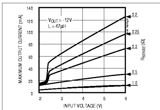
Figure 9b. Maximum Output Current vs. Input Voltage, V_{\text{OUT}} = -12\text{V}
