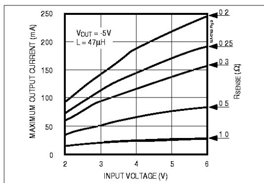
Figure 9a. Maximum Output Current vs. Input Voltage, V_{\text{OUT}} = -5\text{V}
