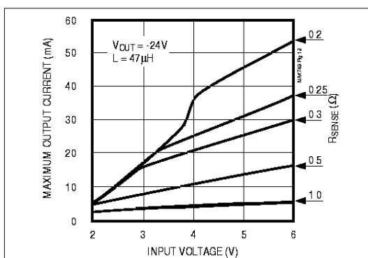
Figure 9d. Maximum Output Current vs. Input Voltage, V_{\text{OUT}} = -24\text{V}
