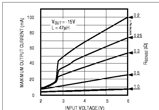
Figure 9c. Maximum Output Current vs. Input Voltage, V_{\text{OUT}} = -15\text{V}
