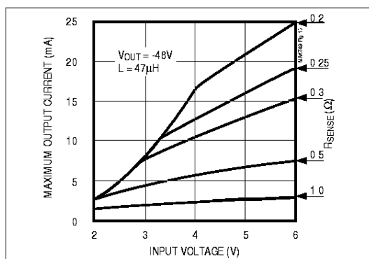
Figure 9e. Maximum Output Current vs. Input Voltage, V_{\text{OUT}} = -48\text{V}
