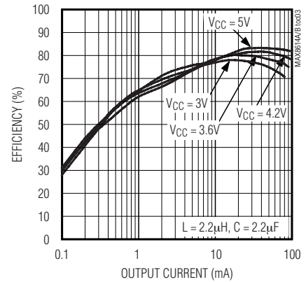
NEGATIVE OUTPUT EFFICIENCY vs. OUTPUT CURRENT
