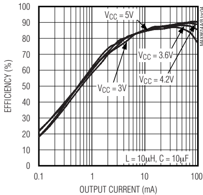
OUTPUT EFFICIENCY vs. OUTPUT CURRENT
