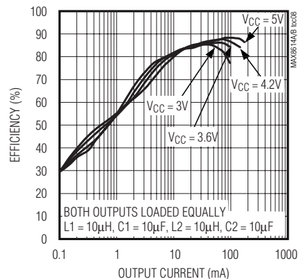
OUTPUT EFFICIENCY vs. OUTPUT CURRENT
