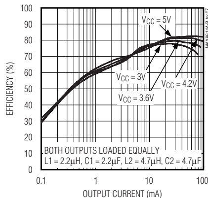
OUTPUT EFFICIENCY vs. OUTPUT CURRENT
