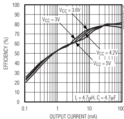
NEGATIVE OUTPUT EFFICIENCY vs. OUTPUT CURRENT
