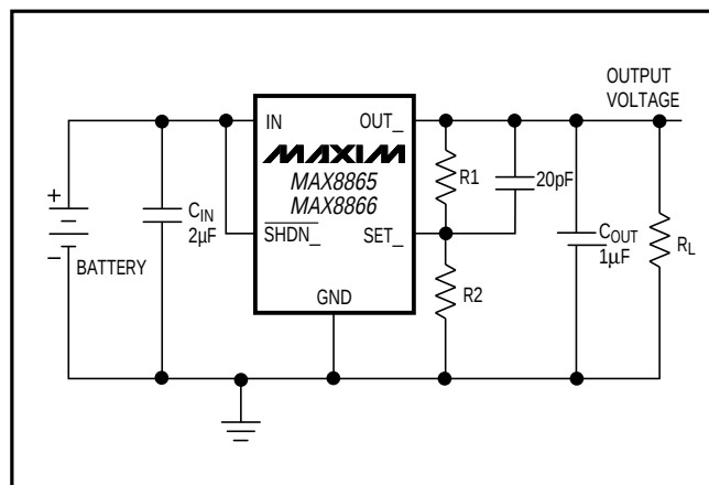
Figure 2. Adjustable Output Using External Feedback Resistors
