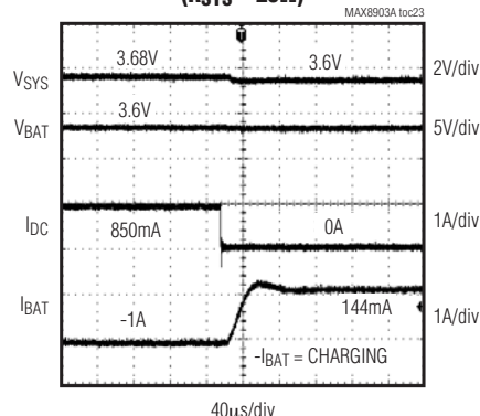
DC DISCONNECT WITH NO USB ( R_{SYS} = 25\Omega )
