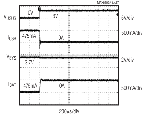
USB SUSPEND
