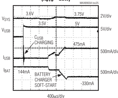
USB CONNECT WITH NO DC ( R_{SYS} = 25\Omega )
