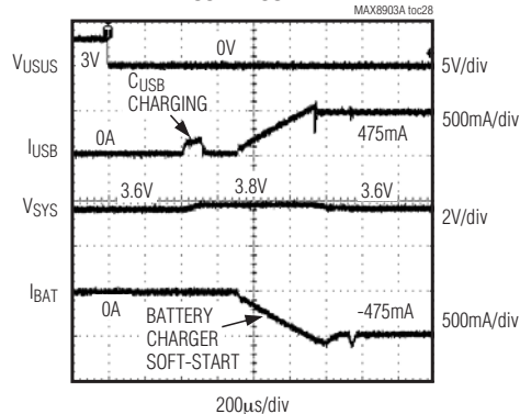
USB RESUME
