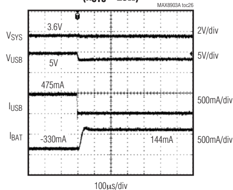
USB DISCONNECT WITH NO DC ( R_{SYS} = 25\Omega )
