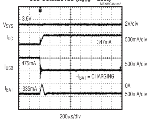
DC CONNECT WITH USB CONNECTED ( R_{SYS} = 25\Omega )
