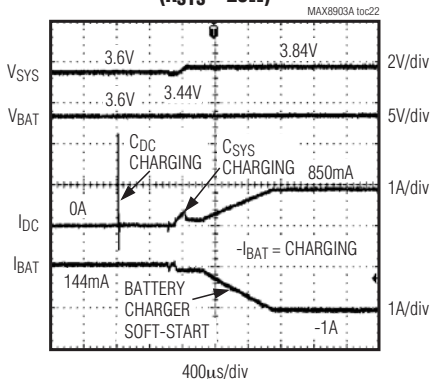
DC CONNECT WITH NO USB ( R_{SYS} = 25\Omega )
