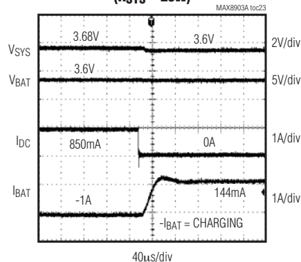
DC DISCONNECT WITH NO USB ( R_{SYS} = 25\Omega )
