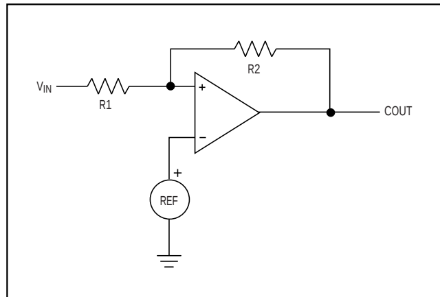
Figure 6. External Hysteresis
