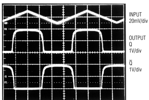
MAX912/MAX913 RESPONSE
