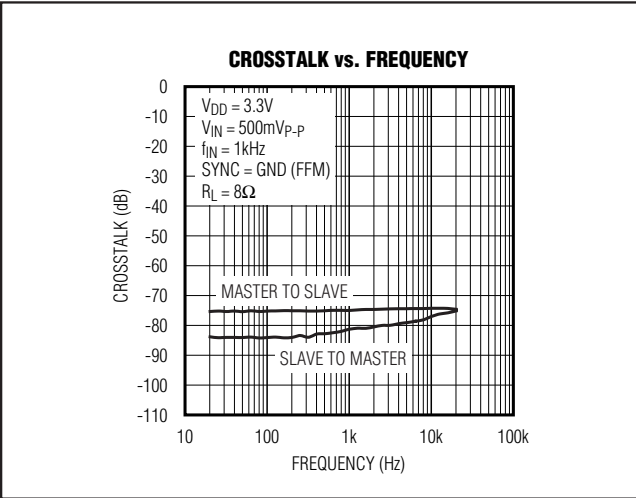
Figure 8. Master-Slave Crosstalk
