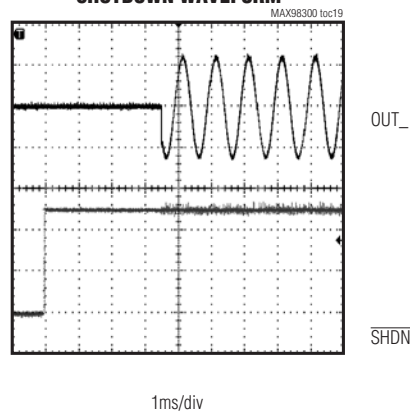
SHUTDOWN WAVEFORM
