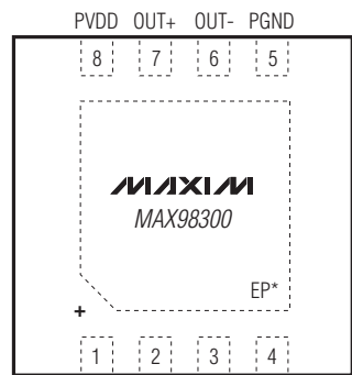
TDFN (2mm x 2mm)
