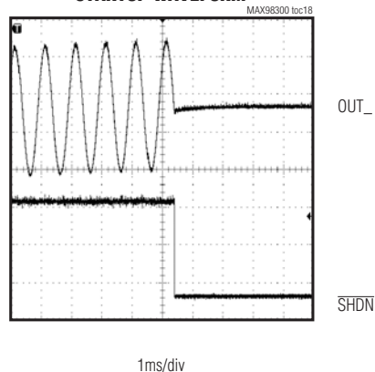
STARTUP WAVEFORM
