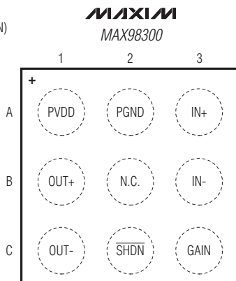
WLP (1.2mm x 1.2mm, 0.4mm pitch)
