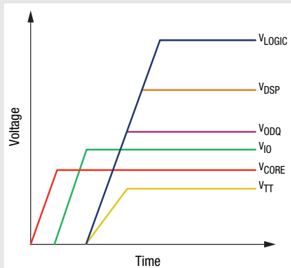
Control Power Up/Down Sequencing with Different Delays and Slopes
