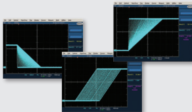
Control Power Up/Down Sequencing with Different Delays and Slopes
