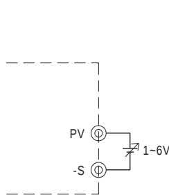
Fig. 3.1 Add on 1~6V external voltage
