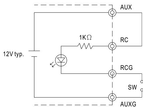
(B)Using internal 12V auxiliary output
