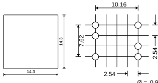
PCB layout (top view)
