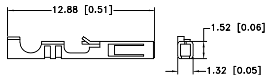
FEMALE CONNECTOR PIN
