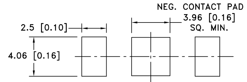
PCB LAYOUT
