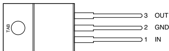
TO-220 (T)
