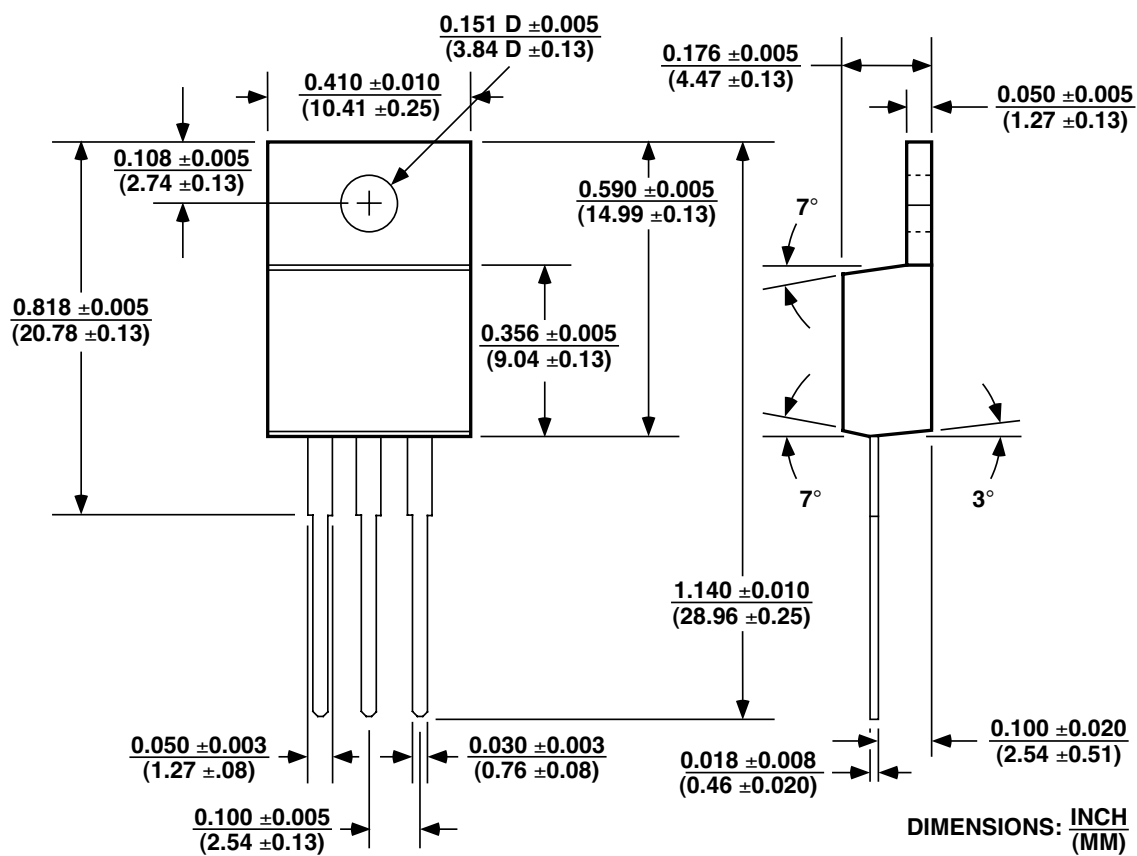
TO-220 (T)
