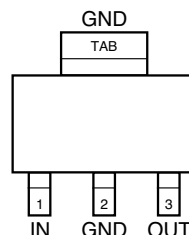
SOT-223 (S)
