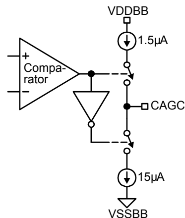
Figure 3. CAGC Pin
