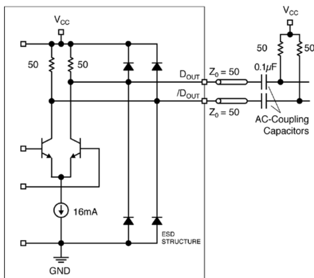
Figure 3. Output Structure
