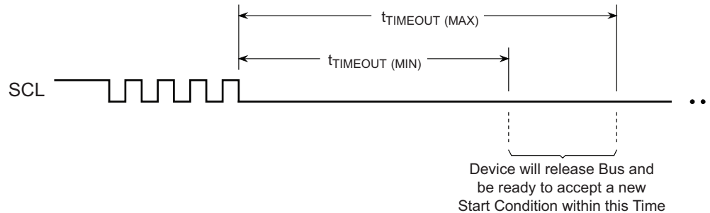
Figure 6-2. SMBus Timeout
