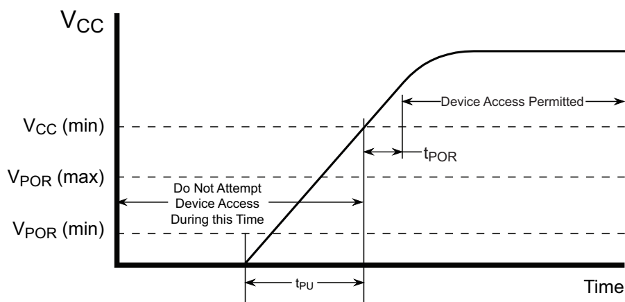
Figure 7-2. Power-Up Timing
