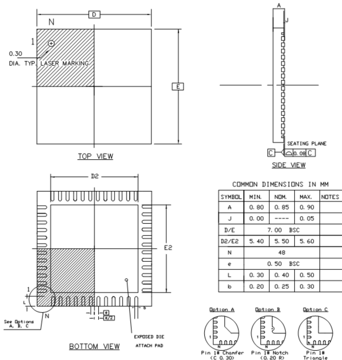
Figure 36-2. QFN-48 Package Drawing
