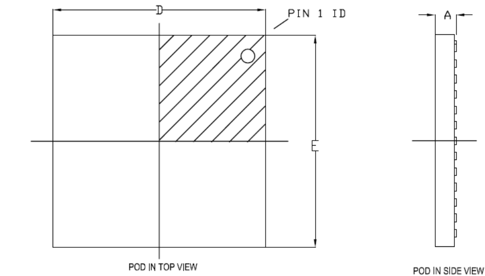
Figure 36-3. TLLGA-48 Package Drawing
