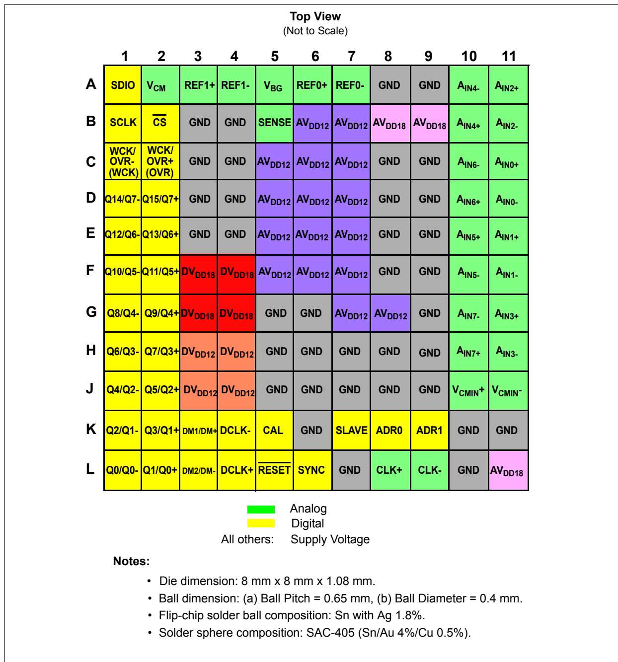
FIGURE 1-2: TFBGA-121 Package. See Table 1-2 for the pin descriptions and Table 1-3 for active and inactive ADC output pins for various ADC resolution modes.
