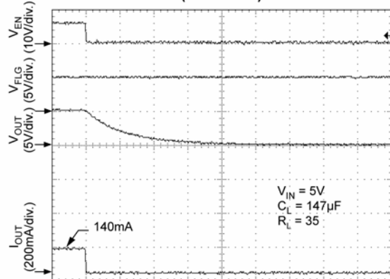
Turn-Off (MIC2026-1)
