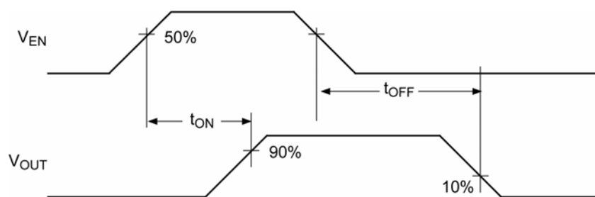
Active-High Switch Delay Time (MIC20x6-1)
