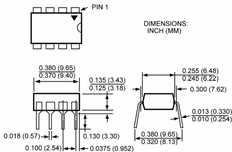
8-Pin DIP (N)
