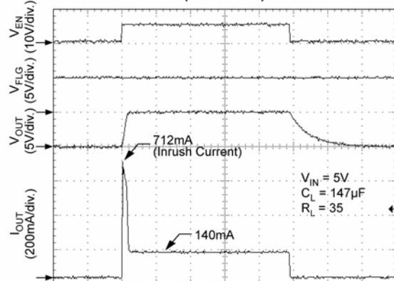
Turn-On/Turn-Off (MIC2026-1)
