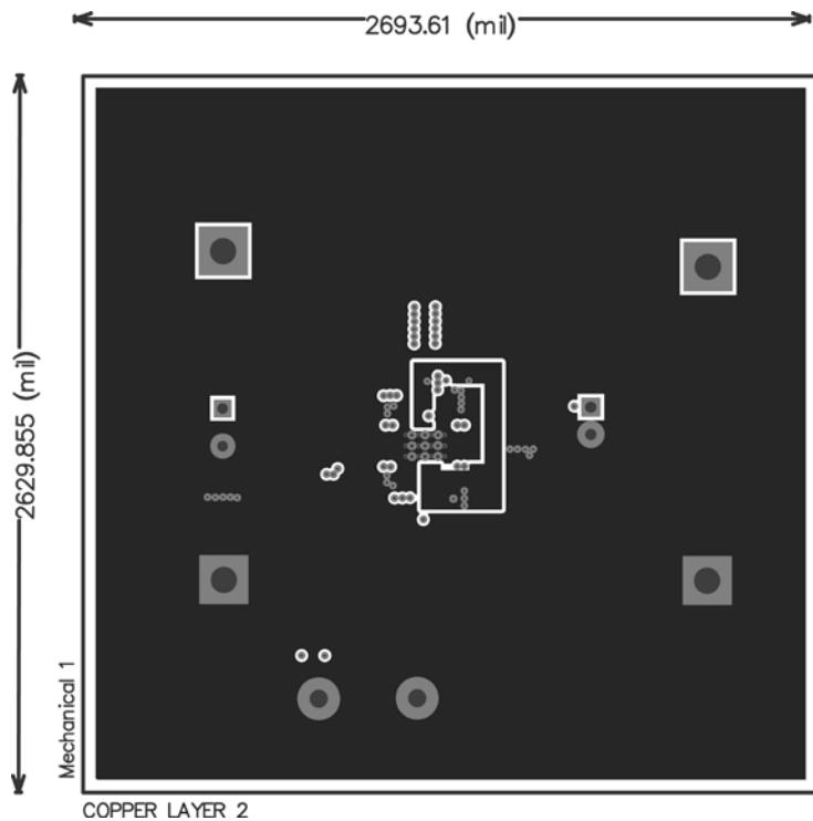
Second Layer
