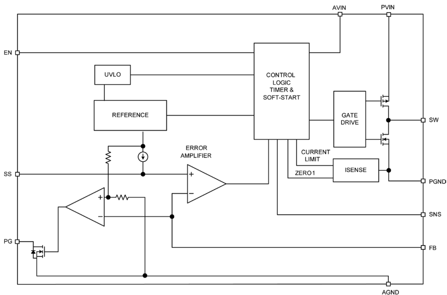
Figure 1. Simplified MIC23603 Functional Block Diagram
