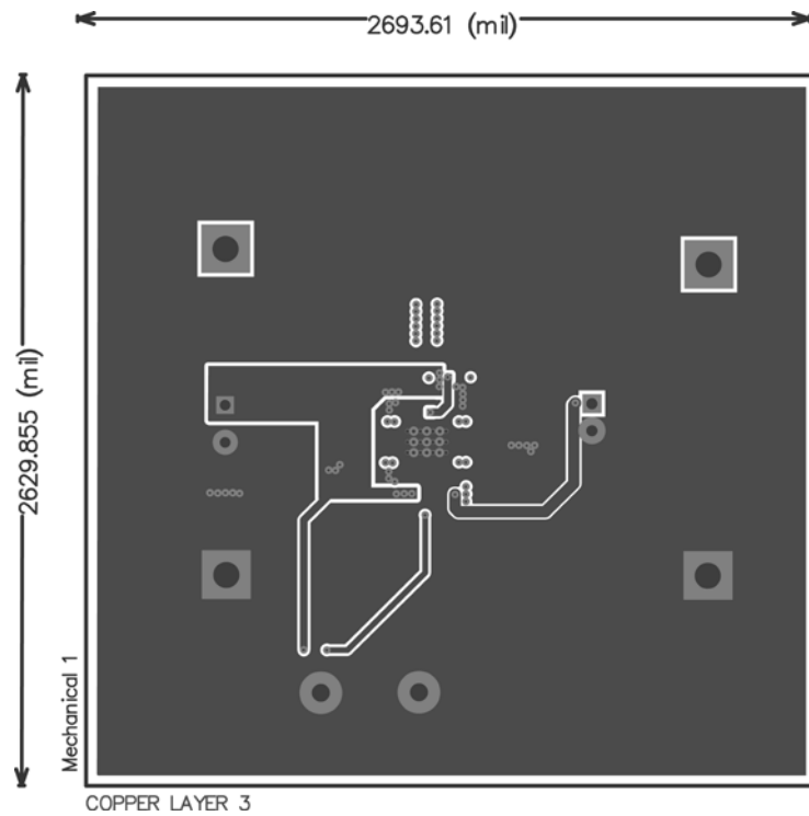
Third Layer
