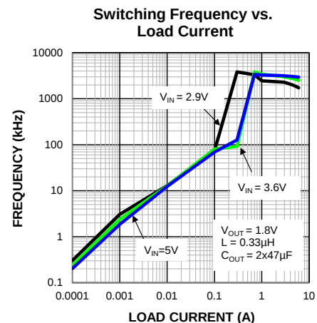
Figure 3. SW Frequency vs. Output Current
