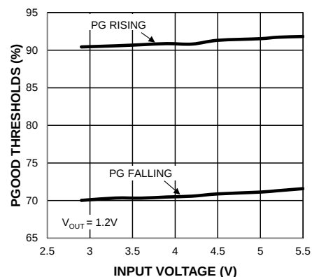
PGOOD Thresholds vs. Input Voltage
