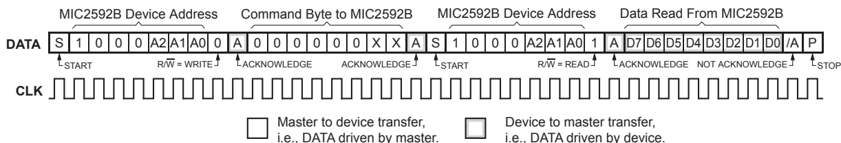
Figure 11. READ_BYTE Protocol
