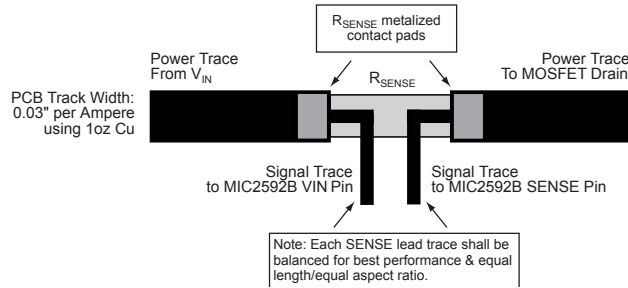
Figure 13. 4-Wire Kelvin Sense Connections for R_{\text{SENSE}}
