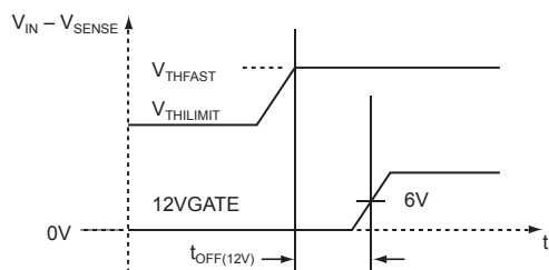
Figure 2. 12V Current Limit Response Timing
