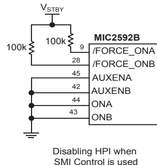
Figure 6. Input Pin Configuration for Disabling HPI/SMI Control
