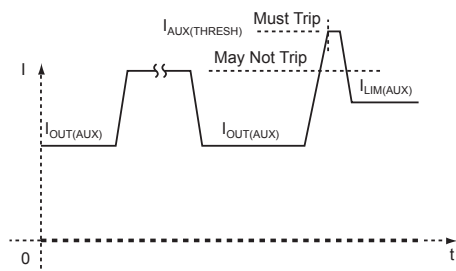
Figure 4. VAUX Current Limit Threshold
