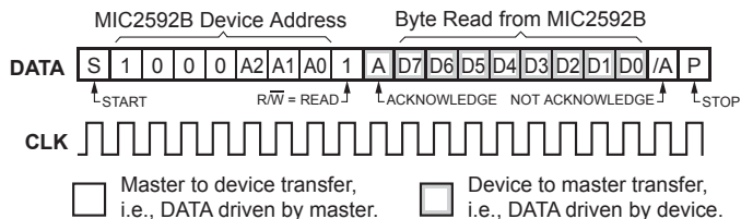
Figure 12. RECEIVE_BYTE Protocol
