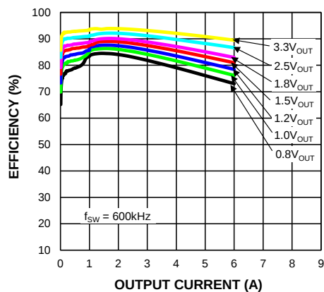
Efficiency ( V_{IN} = 5V ) vs. Output Current (MIC4205-1)
