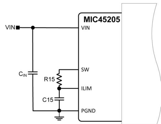
Figure 5. MIC45205 Current-Limiting Circuit
