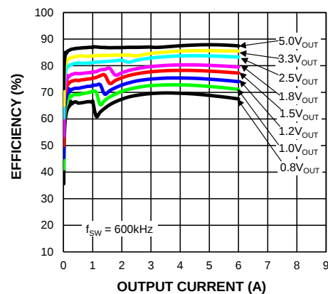
Efficiency ( V_{IN} = 24V ) vs. Output Current (MIC45205-1)
