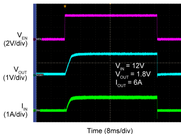
Enable Turn-On/Off
