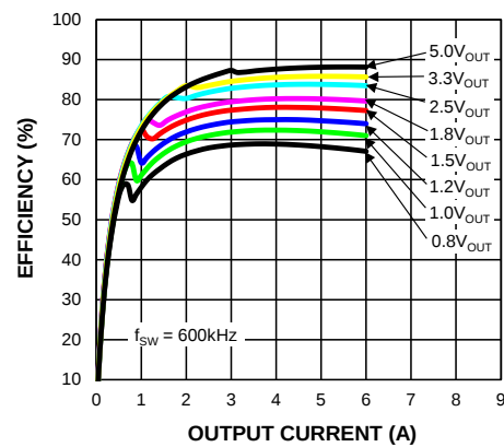
Efficiency ( V_{IN} = 24V ) vs. Output Current (MIC45205-2)
