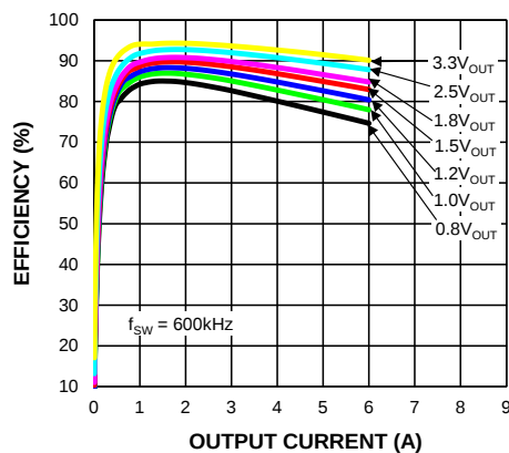
Efficiency ( V_{IN} = 5V ) vs. Output Current (MIC45205-2)
