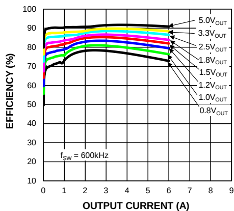
Efficiency ( V_{IN} = 12V ) vs. Output Current (MIC45205-1)
