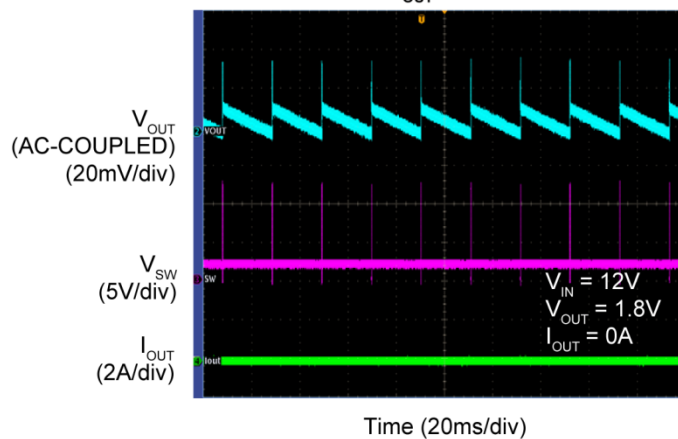
Switching Waveforms – MIC45205-1 ( I_{OUT} = 0A )
