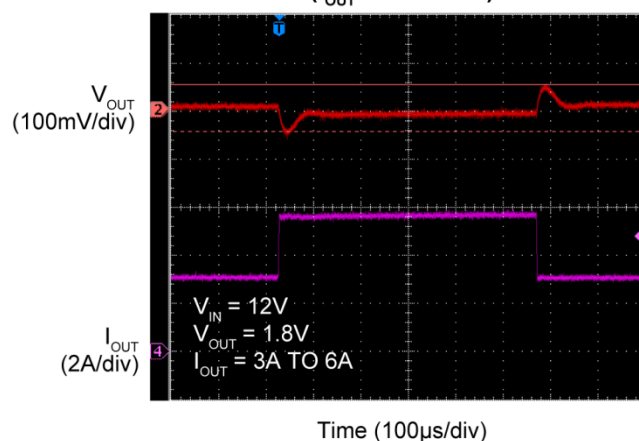
Transient Response – MIC45205-1 ( I_{OUT} = 3A to 6A )
