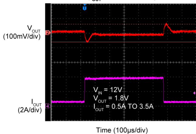
Transient Response – MIC45205-1 ( I_{OUT} = 0.5A to 3.5A )
