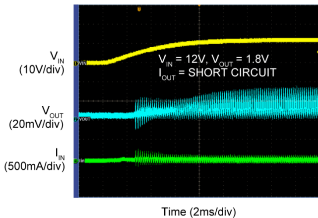
Short Circuit
