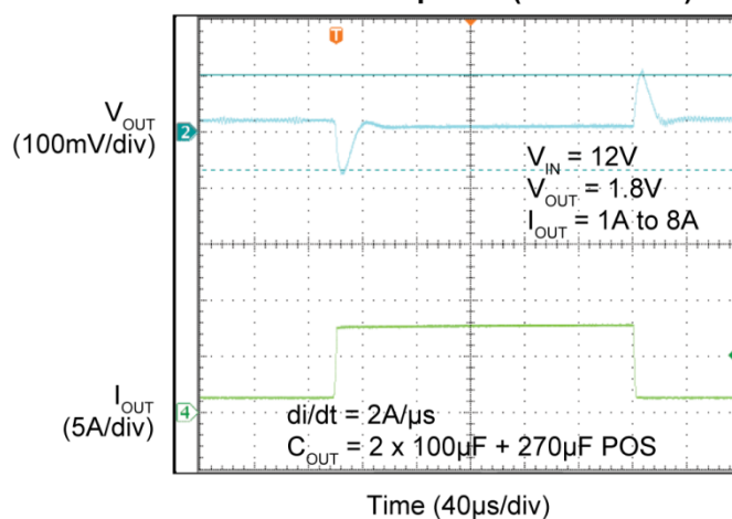
Transient Response (MIC45212-1)
