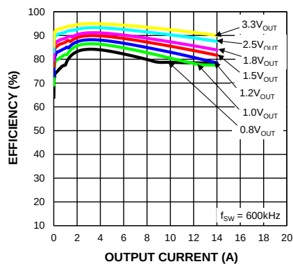
Efficiency vs. Output Current (MIC45212-1, V_{IN} = 5V )
