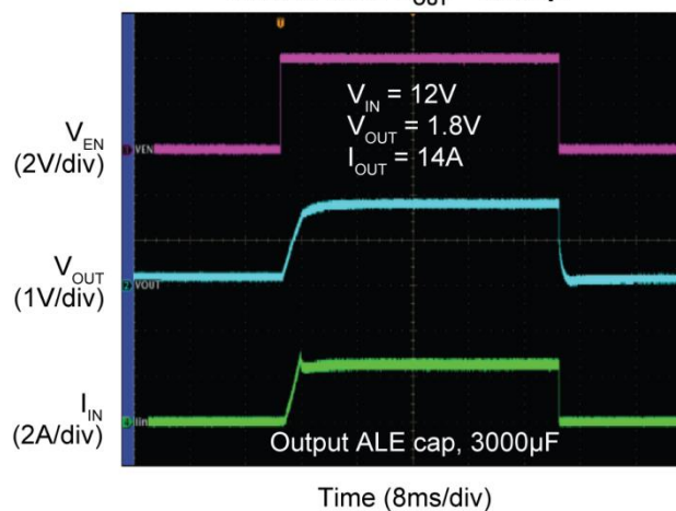
Inrush with C_{OUT} = 3000\mu F
