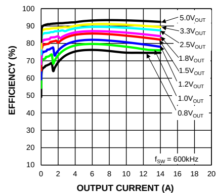
Efficiency vs. Output Current (MIC45212-1, V_{IN} = 12V )
