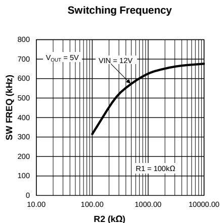
Figure 7. Switching Frequency vs. R2
