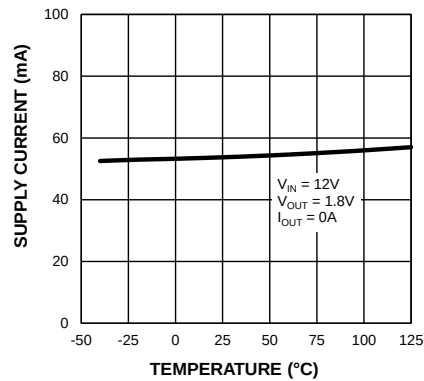
VIN Operating Supply Current vs. Temperature (MIC45212-2)
