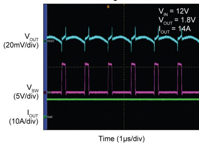
Switching Waveforms
