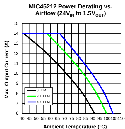
Figure 14. MIC45212 Power Derating vs. Airflow ( 24V_{IN} to 1.5V_{OUT} )
