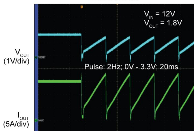
Short Circuit
