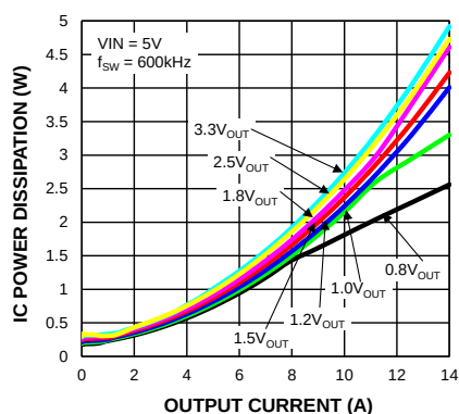
IC Power Dissipation vs. Output Current
