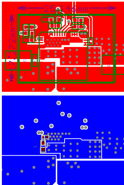
Figure 16. Top And Bottom Layer of a Four-Layer Board
