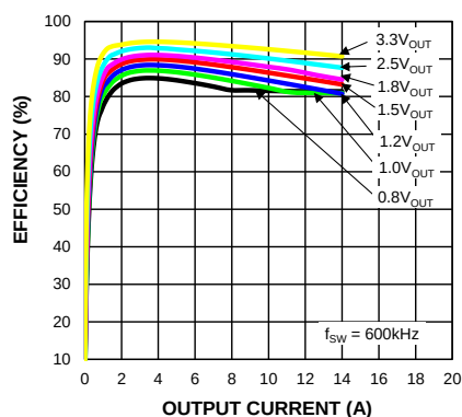
Efficiency vs. Output Current (MIC45212-2, V_{IN} = 5V )
