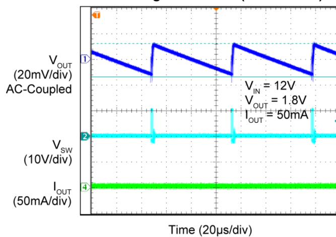
Switching Waveforms (MIC45212-1)
