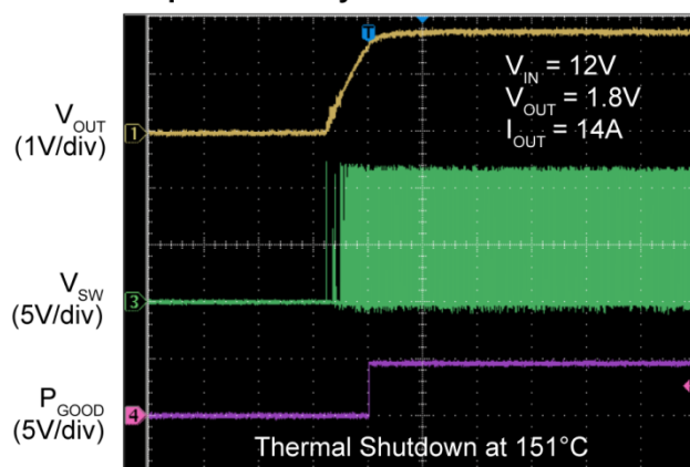
Output Recovery from Thermal Shutdown
