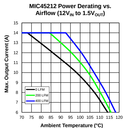
Figure 12. MIC45212 Power Derating vs. Airflow ( 12V_{IN} to 1.5V_{OUT} )
