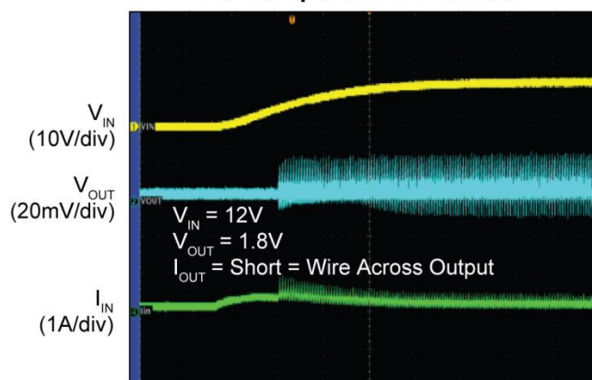
Power-Up Into Short Circuit
