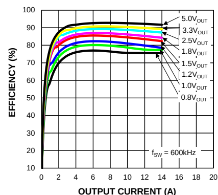
Efficiency vs. Output Current (MIC45212-2, V_{IN} = 12V )
