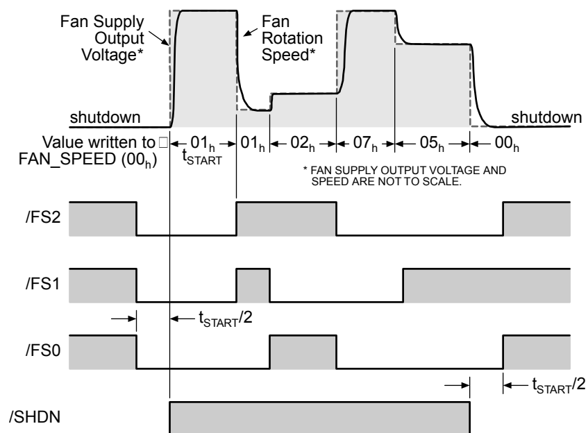
Figure 2. Typical MIC74 Fan-Mode Timing and System Behavior
