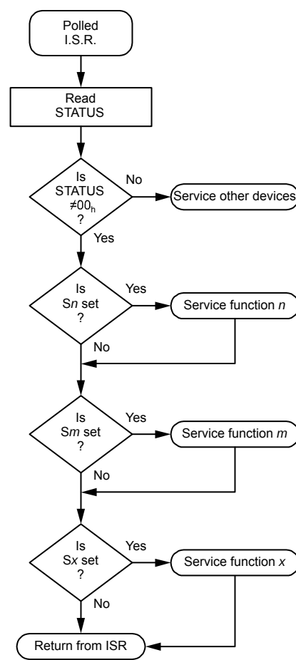
Figure 12: Interrupt Service Routine Without ARA
