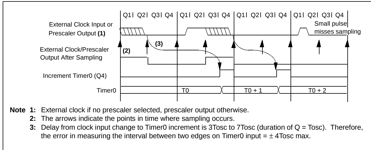
FIGURE 8-5: TIMER0 TIMING WITH EXTERNAL CLOCK
