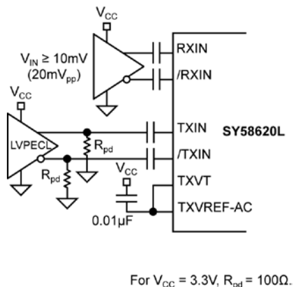
Figure 8b. LVPECL Interface (TX AC-Coupled/RX AC-Coupled)
