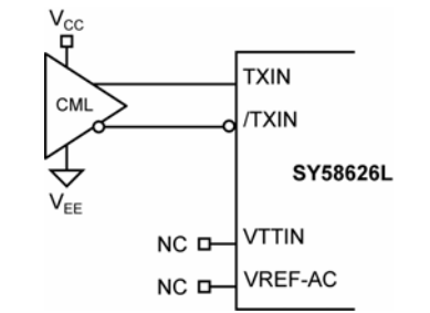
Figure 6c. CML Interface (DC-Coupled)
