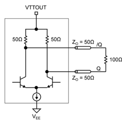
Figure 7a. CML DC-Coupled Termination
