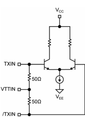
Figure 5a. Simplified Differential Input Stage
