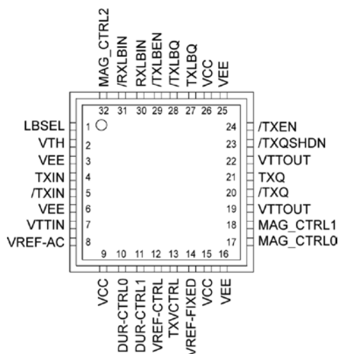
32-Pin QFN
