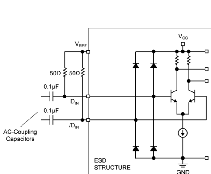
Figure 2. Input Structure
