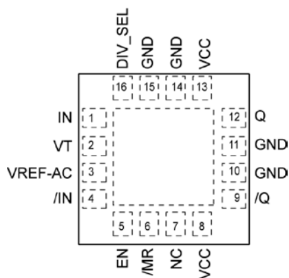
16-Pin QFN
