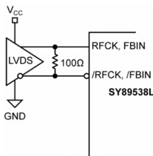
Figure 11e. LVDS (DC-Coupled)
