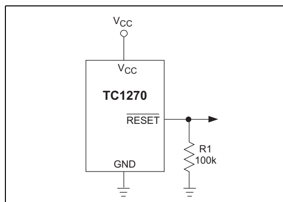
FIGURE 3-2: Ensuring \overline{\text{RESET}} Valid to V_{CC} = 0V
