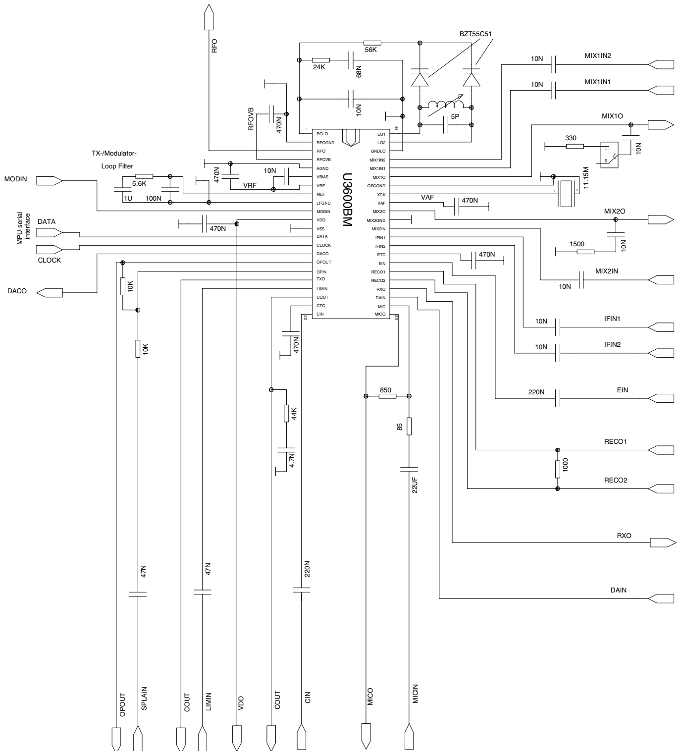
Figure 8-1. Test Circuit
