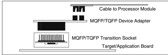
FIGURE 6: MQFP/TQFP TWO-PART TRANSITION SOCKET
