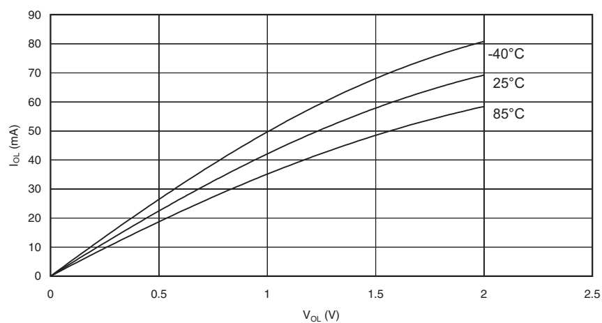
Figure 149. I/O Pin Sink Current vs. Output Voltage ( V_{CC} = 5V )
