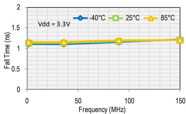
Fall Time
