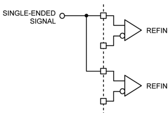
Figure 2. Single-Ended Signal
