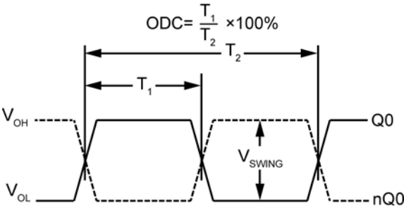
Figure 5. Duty Cycle Timing
