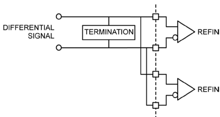
Figure 1. Differential Signal
