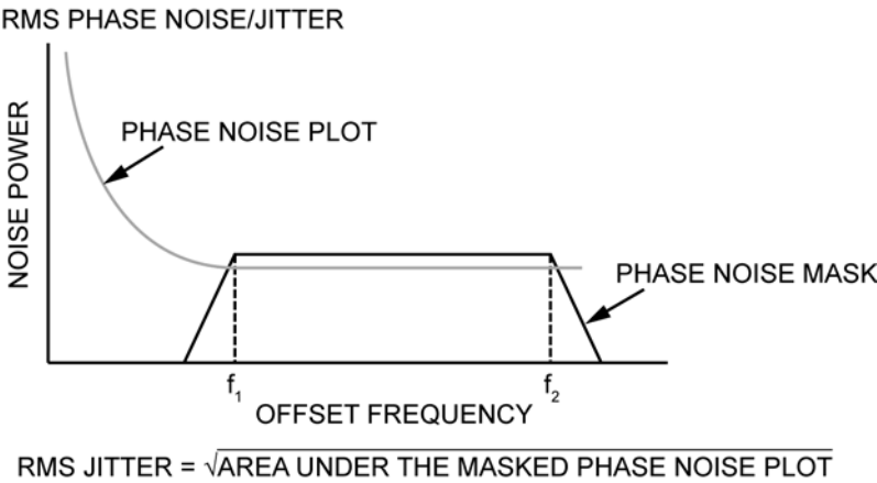
Figure 7. RMS Phase/Noise/Jitter
