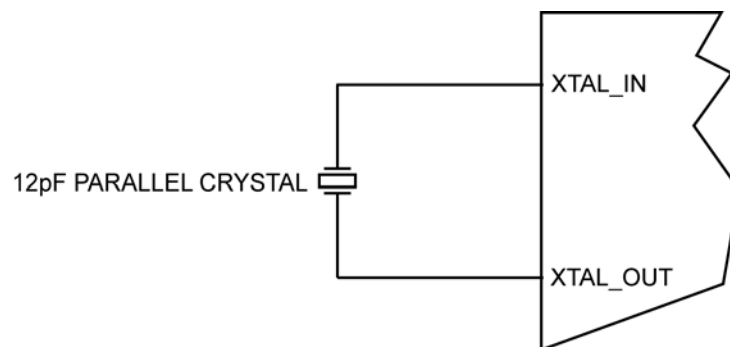
Figure 12. Crystal Input Interface
