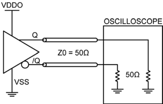
Figure 9. HCSL Output Load and Test Circuit
