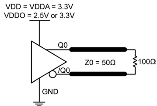
Figure 10. LVDS Output Load and Test Circuit
