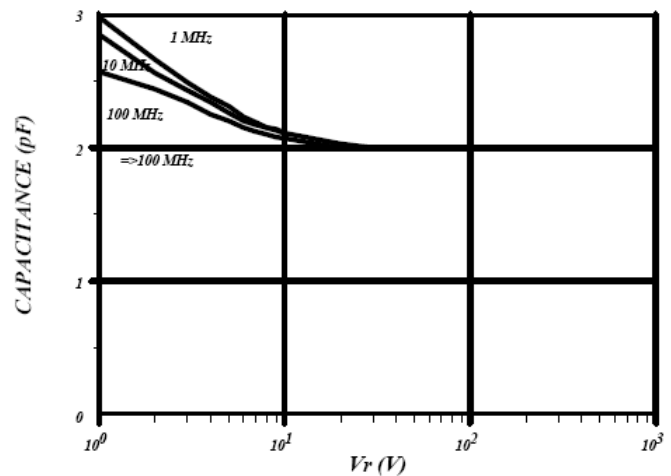
UM7200 TYPICAL
