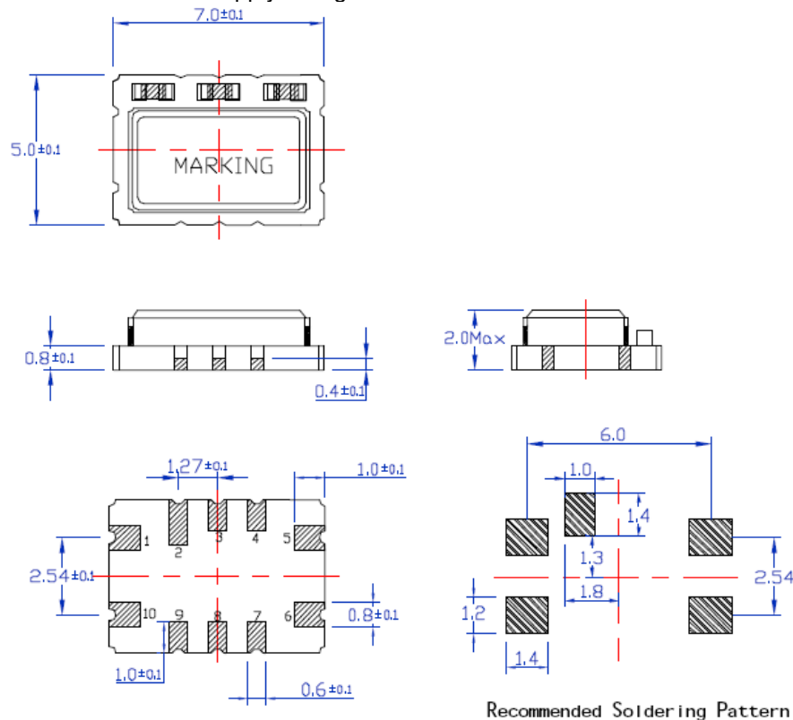
Figure 2, Package drawing
