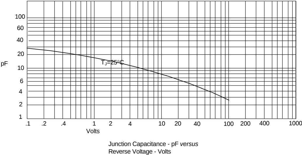
Figure 3 Junction Capacitance
