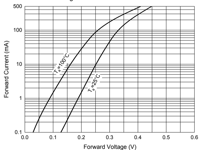
Fig. 1 - Forward Characteristics
