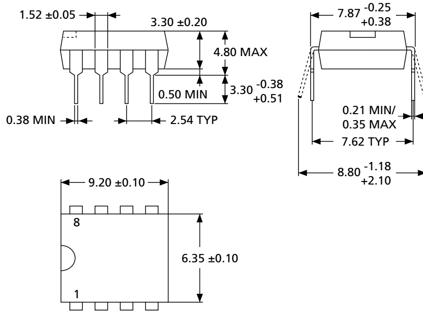
Figure 29: PDIP8 300mils Body Width
