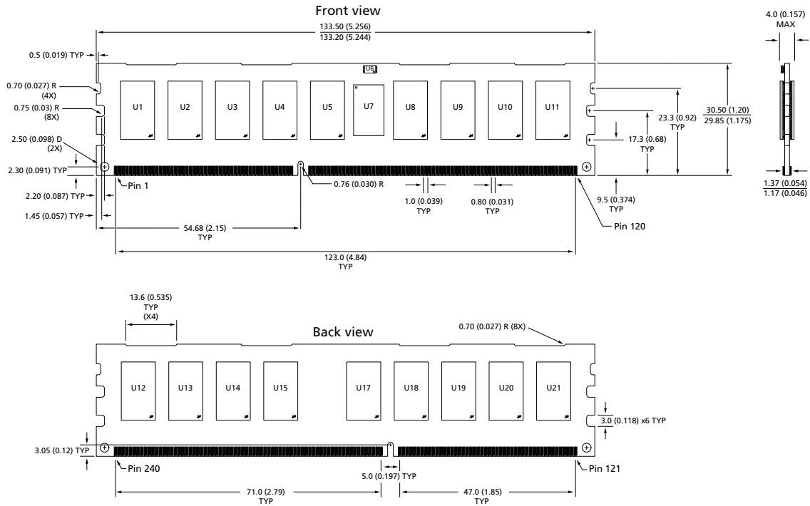
Figure 3: 240-Pin DDR3 RDIMM
