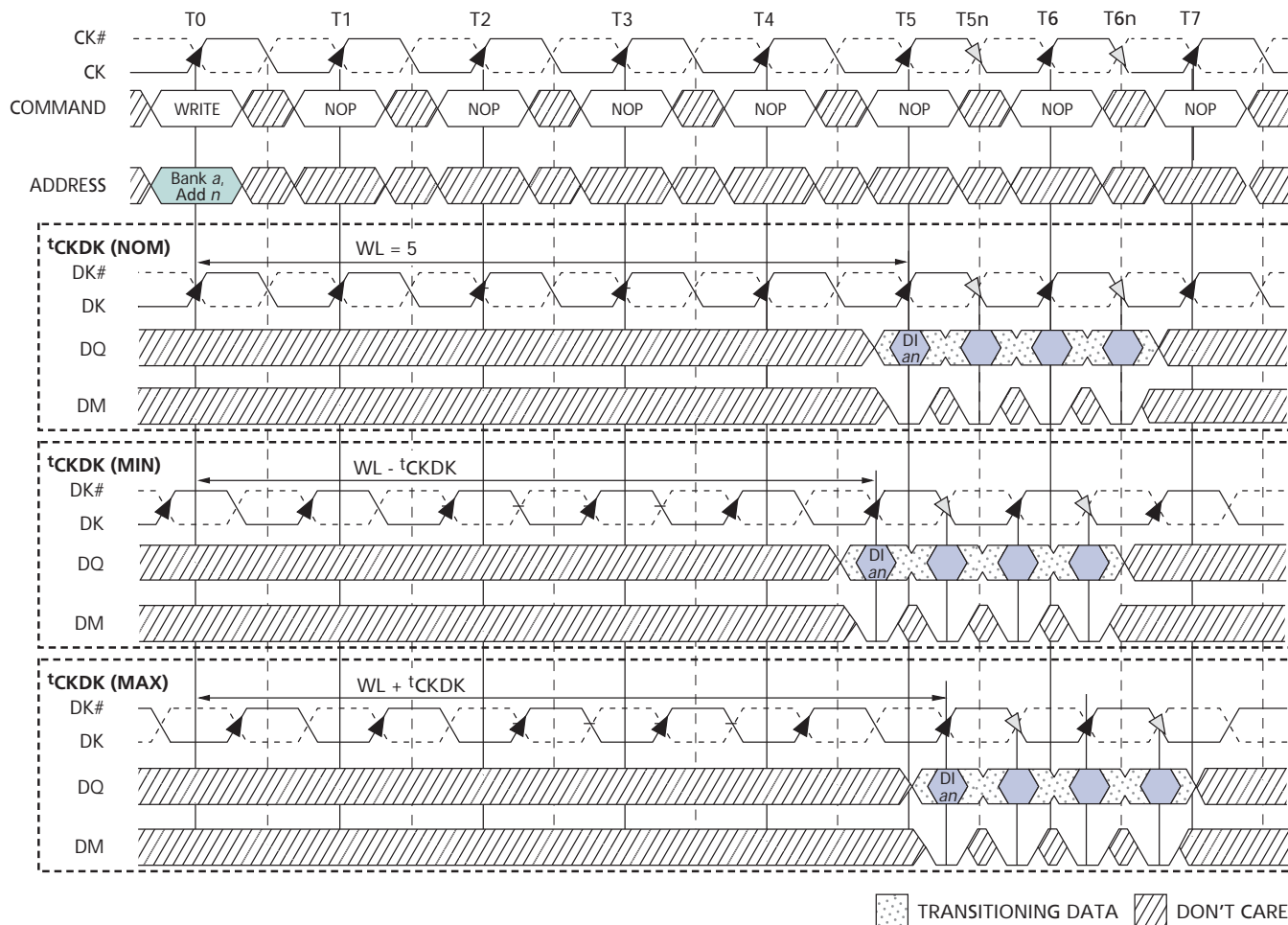
Figure 19: WRITE Burst
