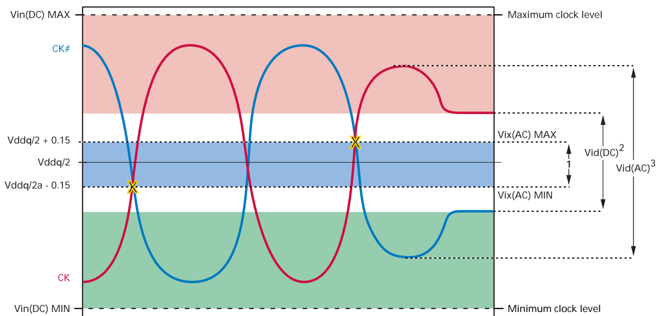
Figure 8: Clock Input
