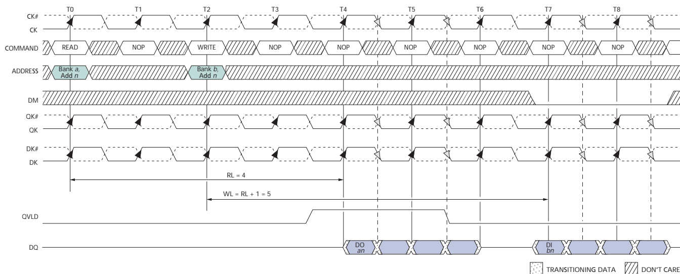
Figure 27: READ-to-WRITE
