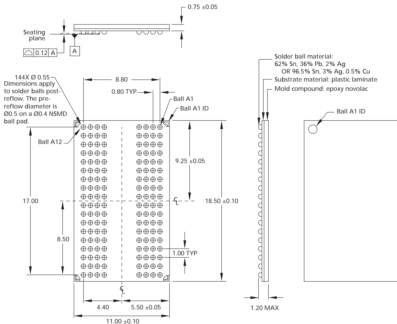
Figure 7: 144-Ball FBGA
