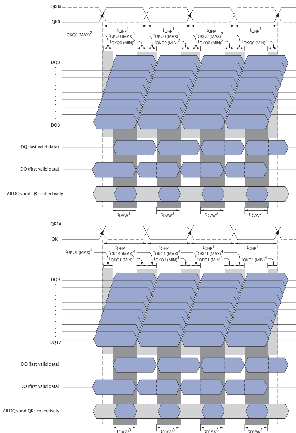
Figure 29: Read Data Valid Window for x18 Device
