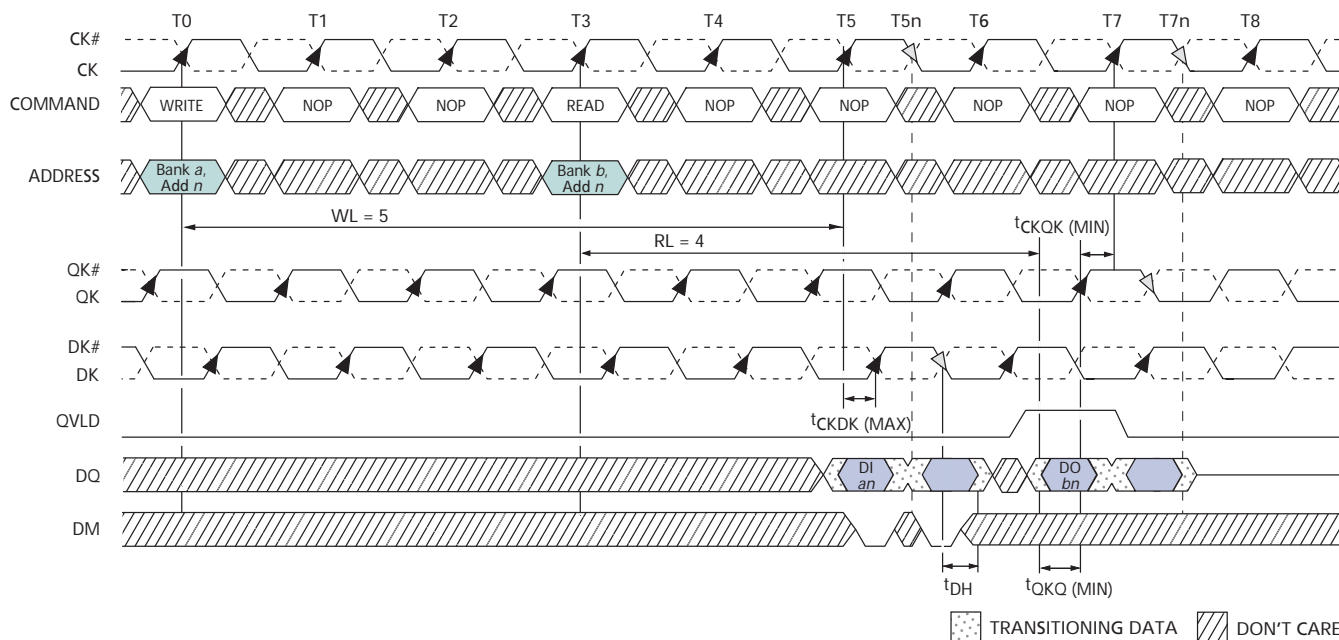
Figure 22: WRITE-to-READ (Separated by Two NOPs)
