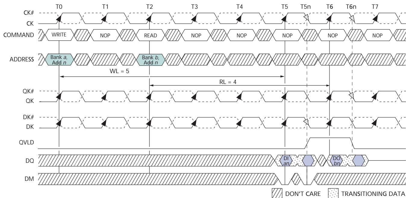
Figure 21: WRITE-to-READ
