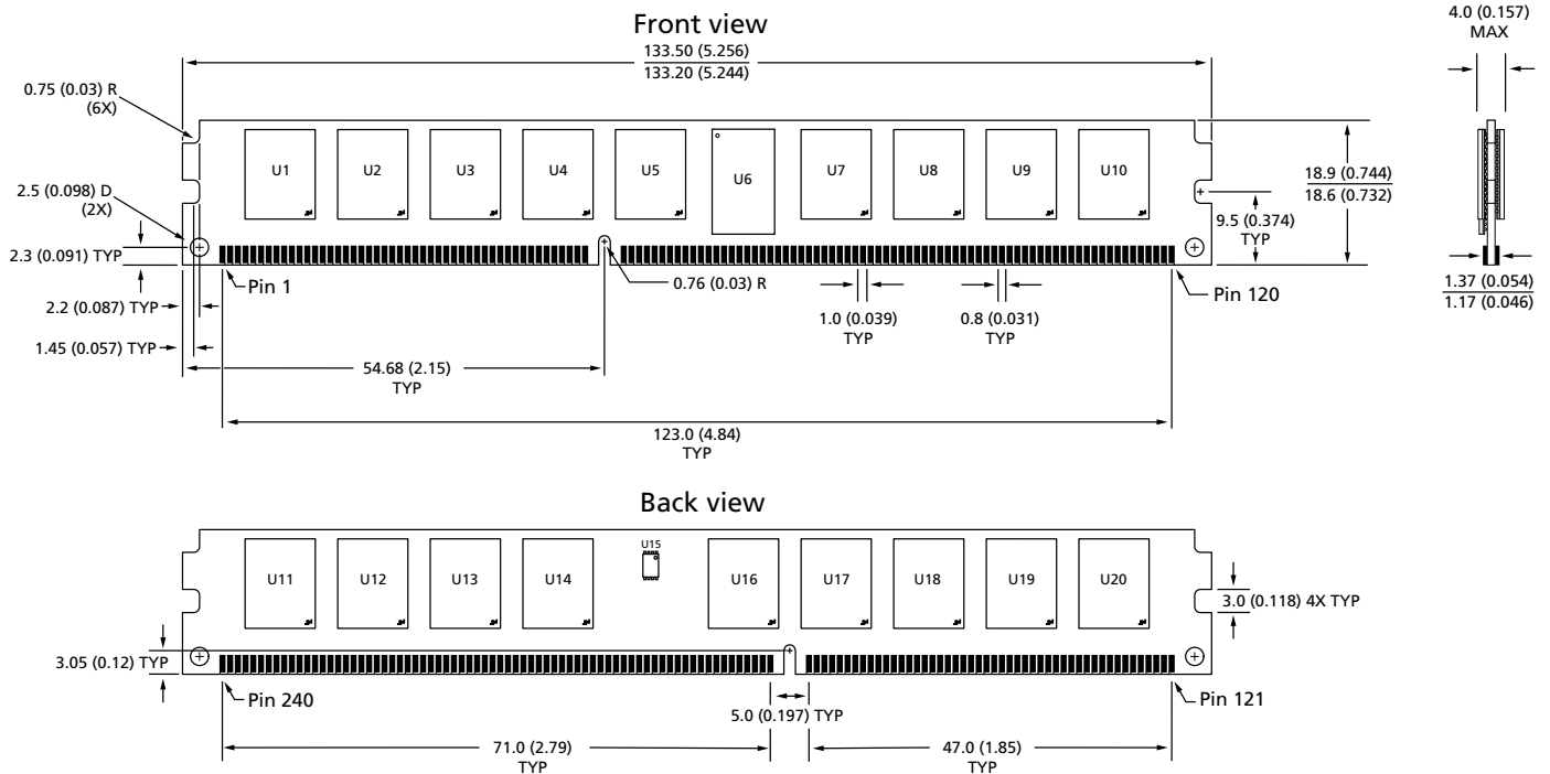
Figure 3: 240-Pin DDR3 VLP RDIMM
